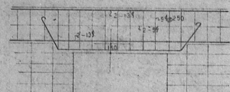
2階 窓上配筋図 S = 30
